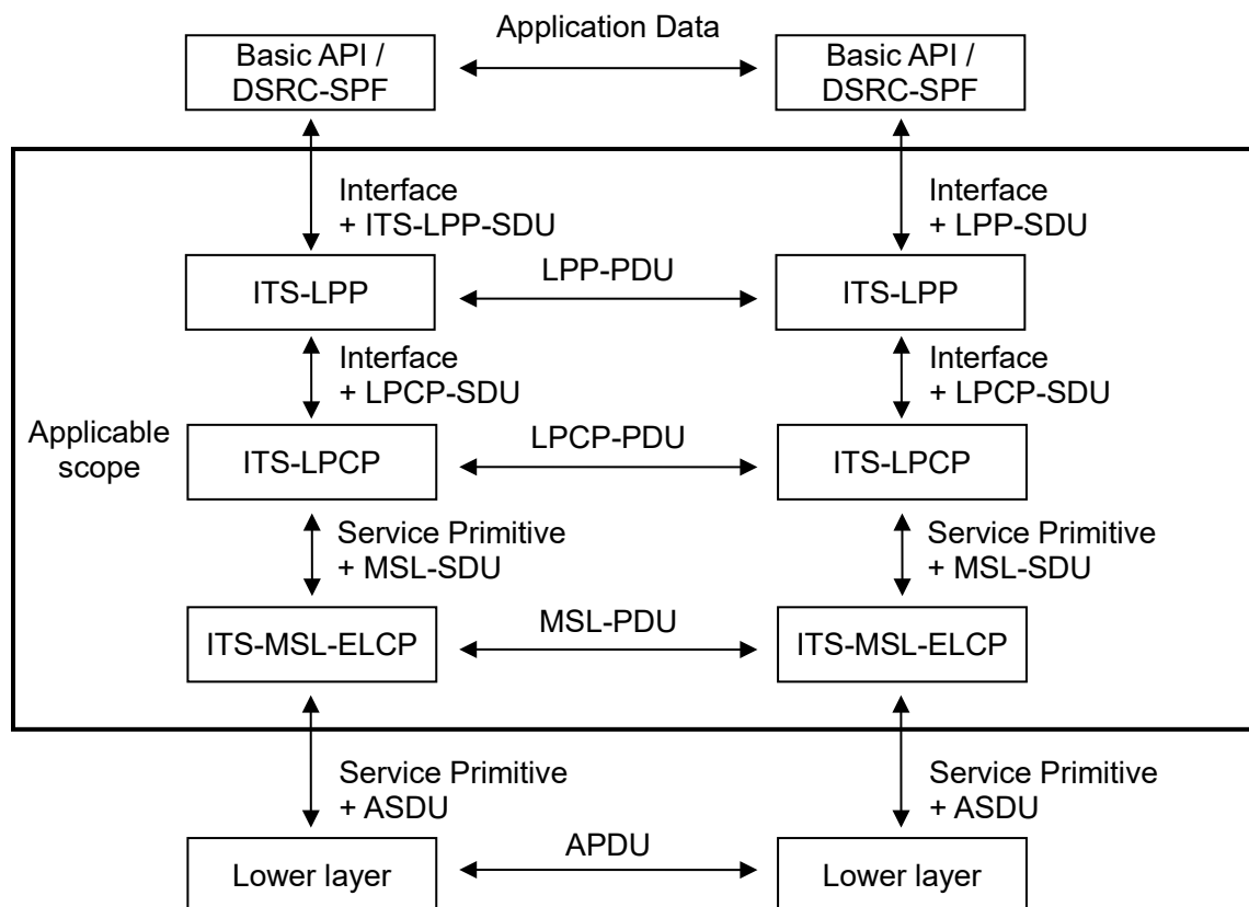
Figure 2.1-1 Overview of the Service Interface and the Protocols of the ITS-MSL
