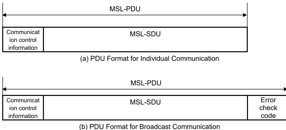
Figure 3.1-8 Configuration of the MSL-PDU (ARIB STD-T120)
