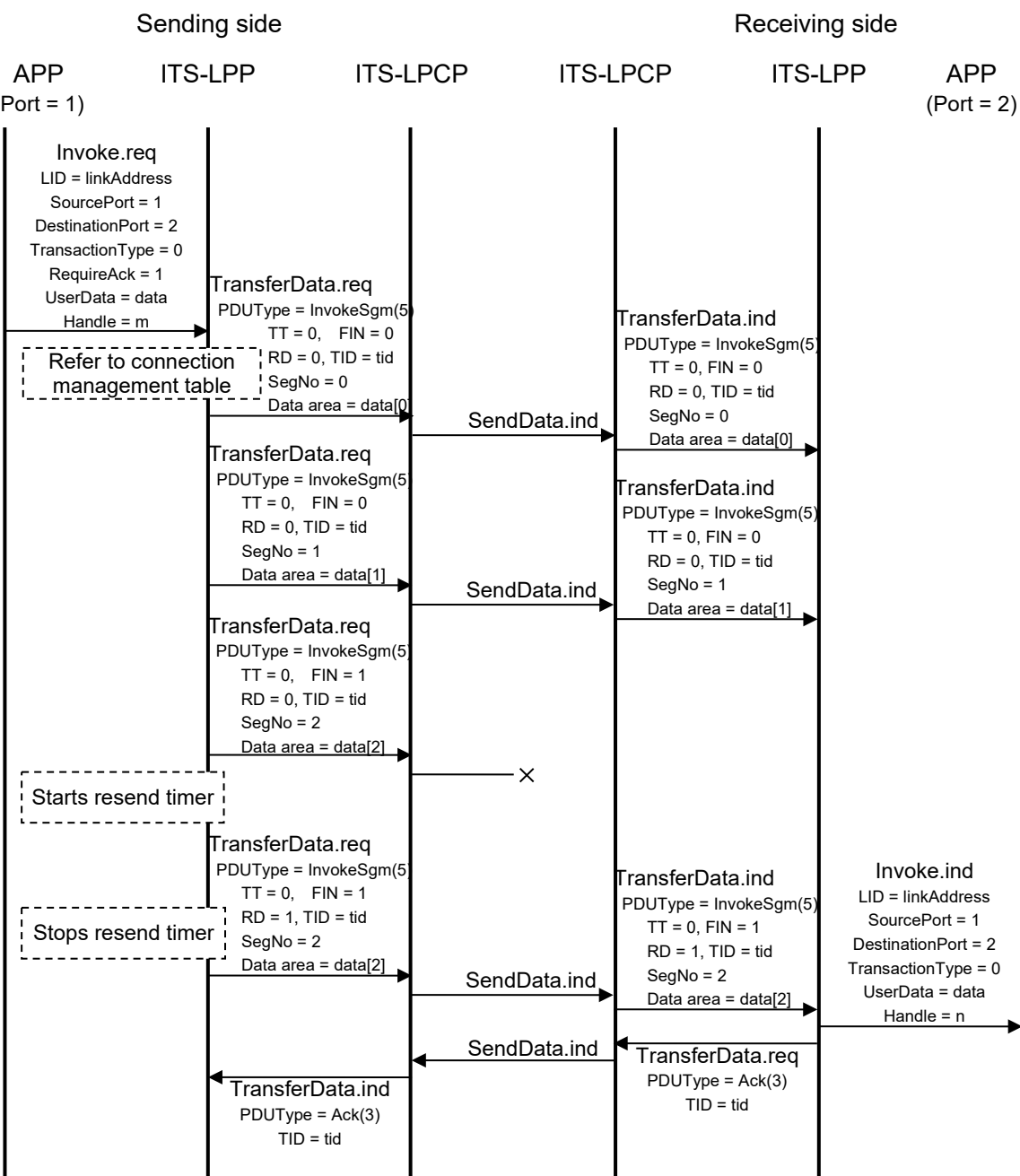
Figure 3.3-22 Example of Segmentation/re-assembly Process
