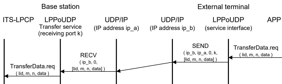
Figure 3.3-32 TransferData.req Sequence
