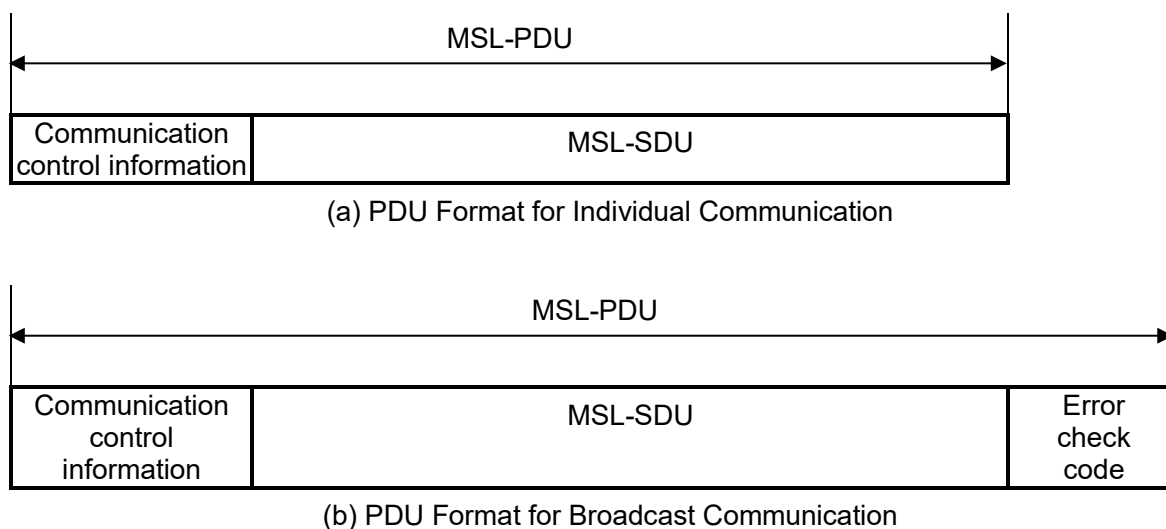
Figure 3.1-6 Configuration of the MSL-PDU (ARIB STD-T104)
