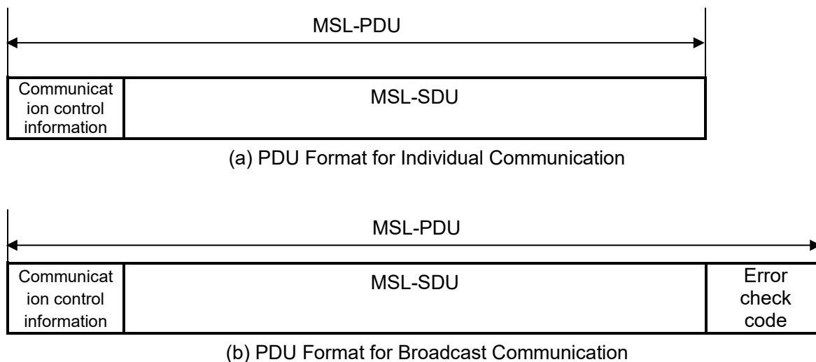
Figure 3.1-7 Configuration of the MSL-PDU (ARIB STD-T109)
