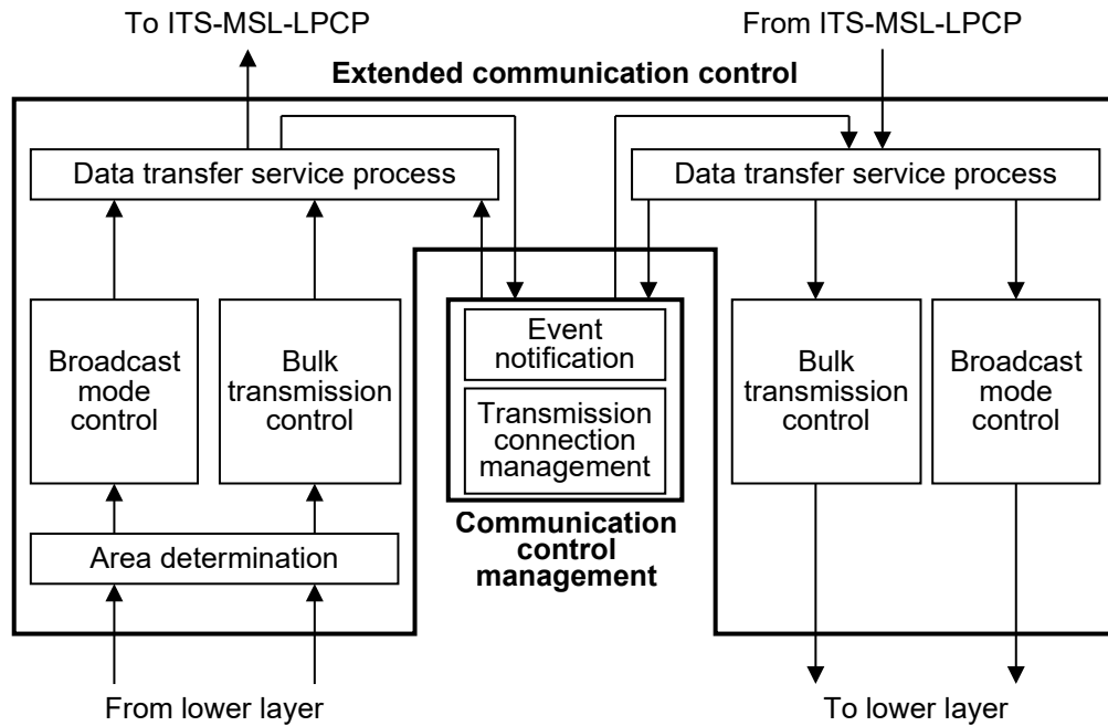
Figure 3.1-1 ITS-MSL-ELCP Entity Configuration of Upper Layer Servers
