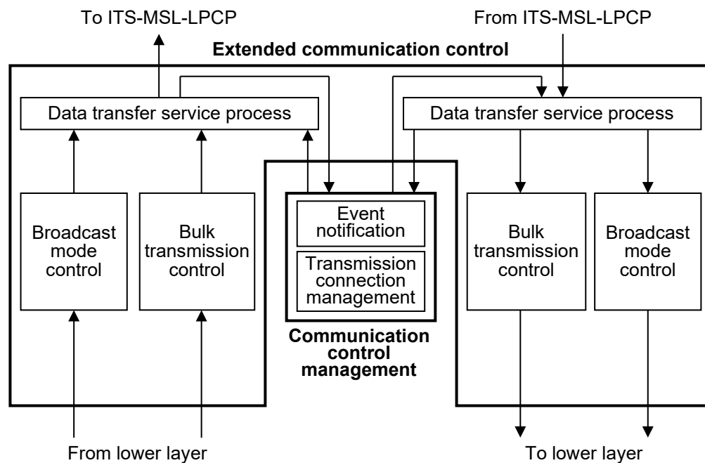
Figure 3.1-2 ITS-MSL-ELCP Entity Configuration of Mobile Stations
