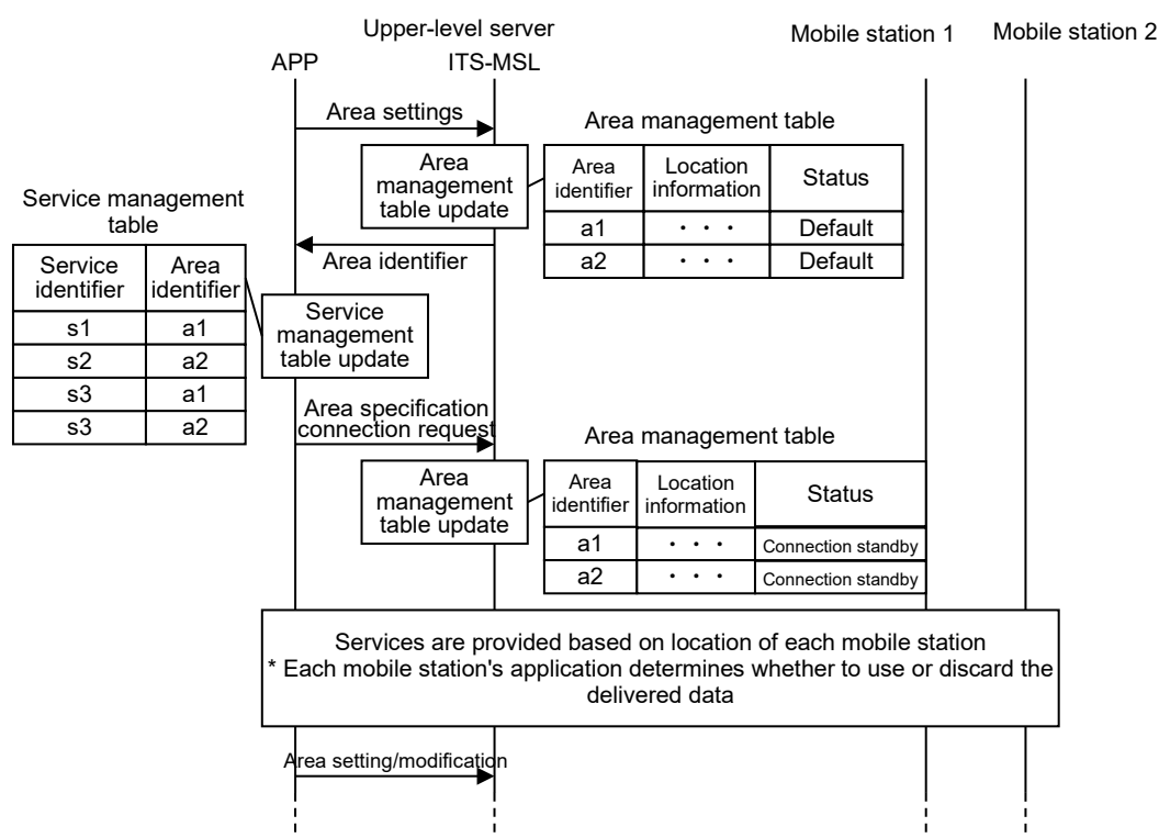
Figure D.7-2 Example of Management Procedure for Services and Service Provision Areas
