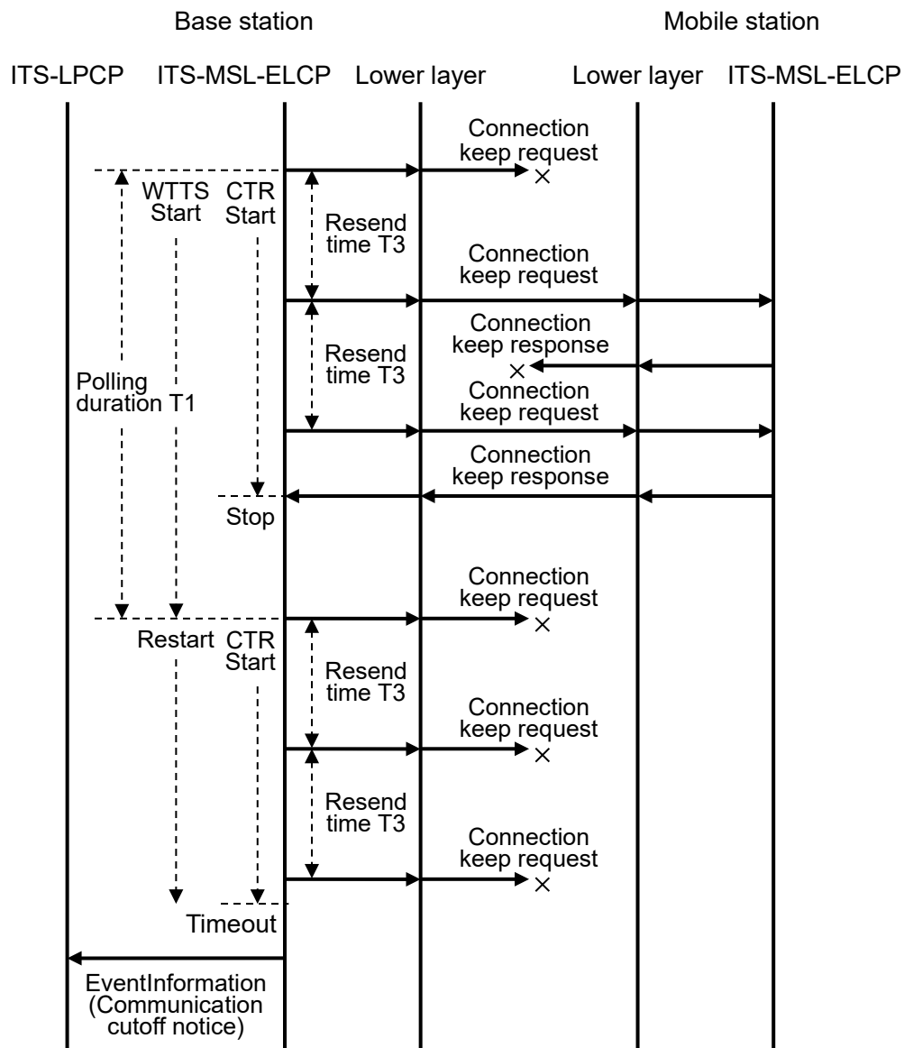
Figure 3.1-15 Example of Resend Control Procedure of Connection Keep Request
