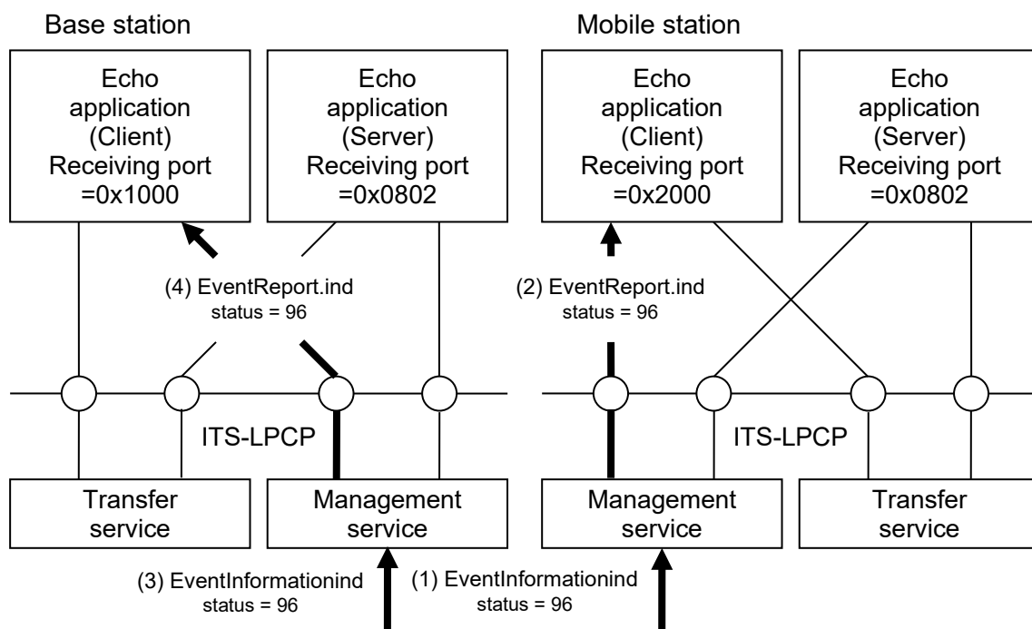
Figure 3.2-10 Initial Set up Operation (connection notice)
