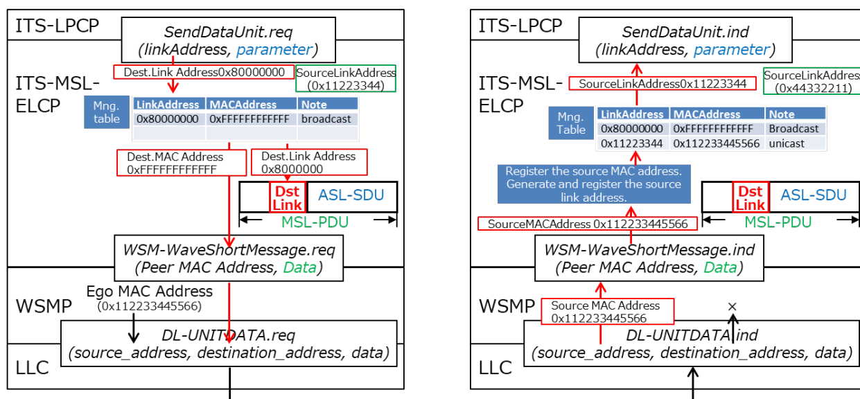
Figure H-1 Example of an Address Management Table
