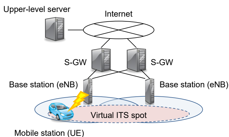
Figure D.1-1 Conceptual Image of Application of ITS-MSL Using LTE-Advanced
