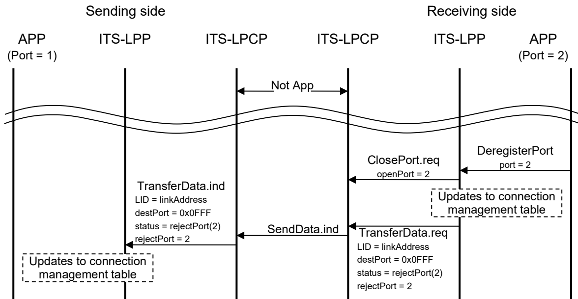
Figure 3.3-27 Example of Accept Port Deletion Procedure
