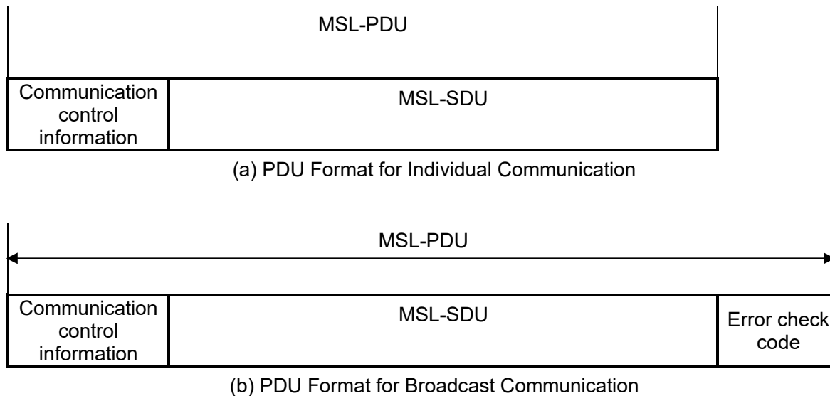
Figure 3.1-5 Configuration of the MSL-PDU (IEEE 802.11/IEEE 802.11bd)
