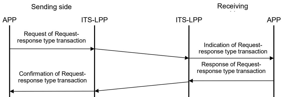
Figure 3.3-4 Example of Request-response Type Transaction Service
