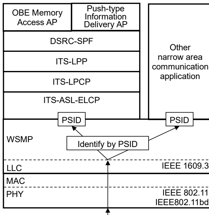
Figure 2.2-2 Identification of the Destination Application in IEEE 802.11/IEEE 802.11bd
