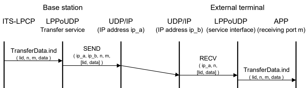
Figure 3.3-34 TransferData.ind Sequence
