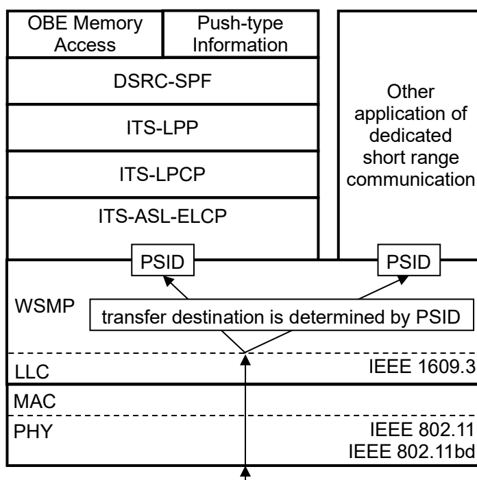
Figure C.1-1 Identification of connection for IEEE 802.11/IEEE 802.11bd
