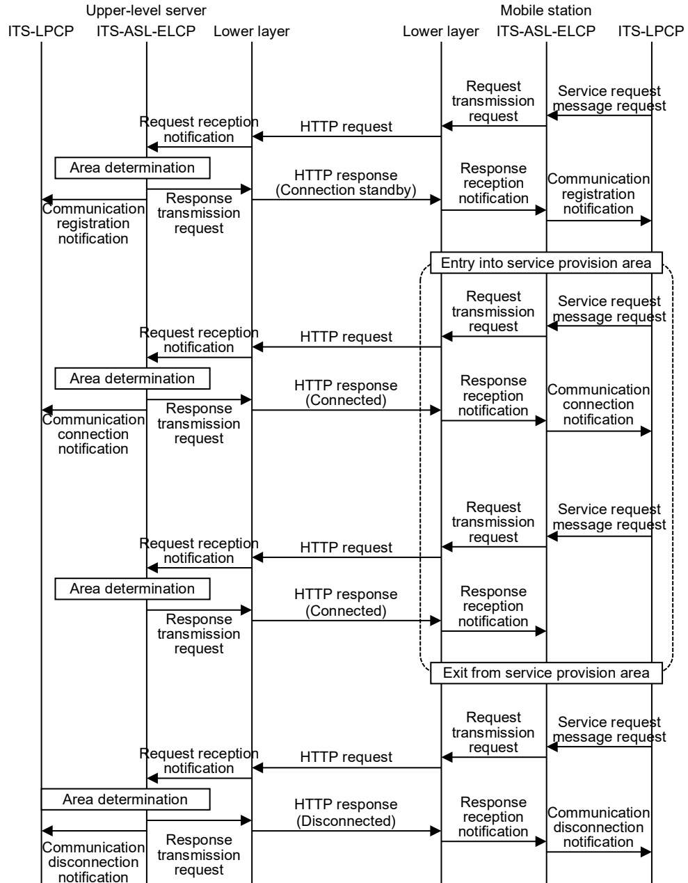
Figure 3.1-18 Example of Communication Connection Procedure
