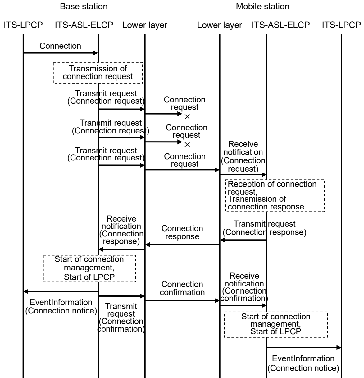
Figure 3.1-13 Example of Communication Connection Procedure
