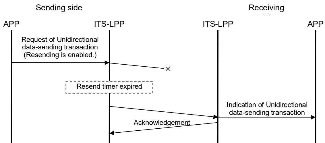
Figure 3.3-5 Example of Data Resending
