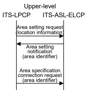
Figure 3.1-17 Example of Area Setting Procedure
