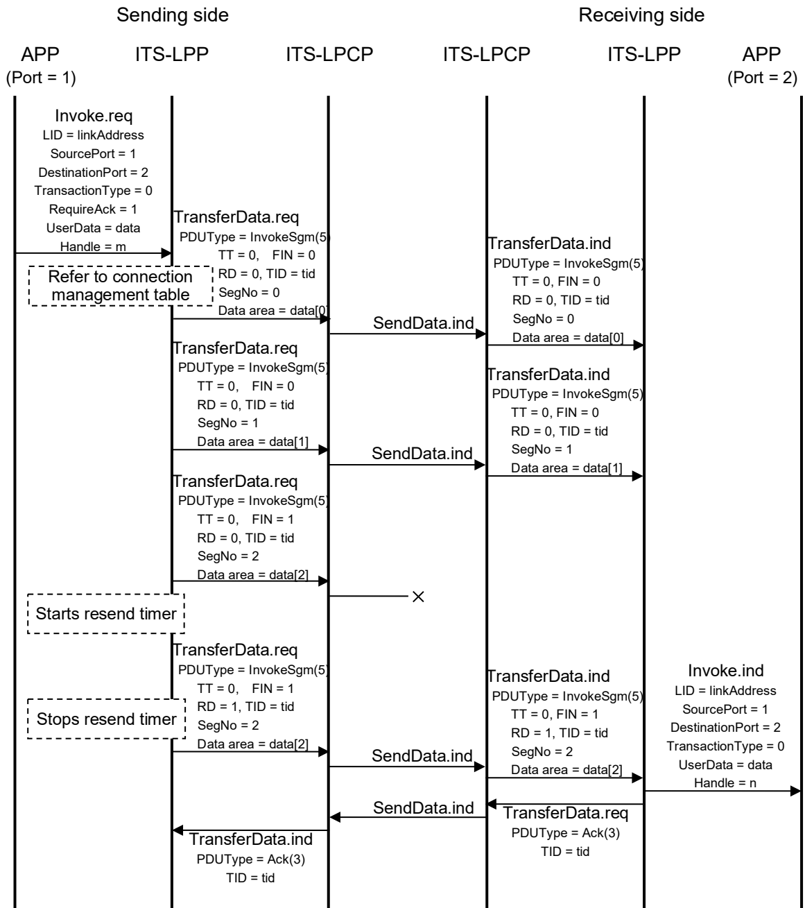
Figure 3.3-22 Example of Segmentation/re-assembly Process
