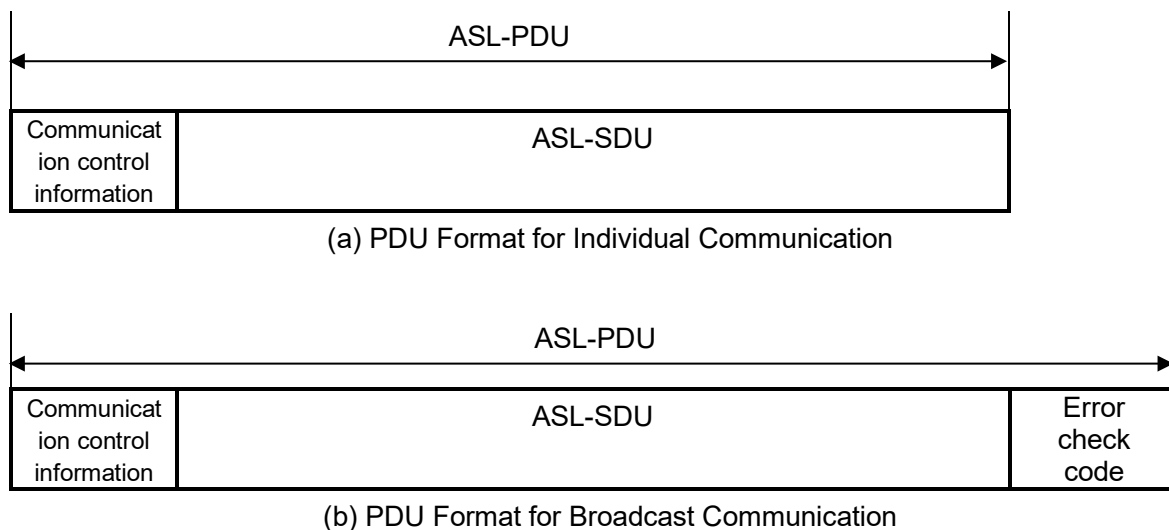
Figure 3.1-8 Configuration of the ASL-PDU (ARIB STD-T120)
