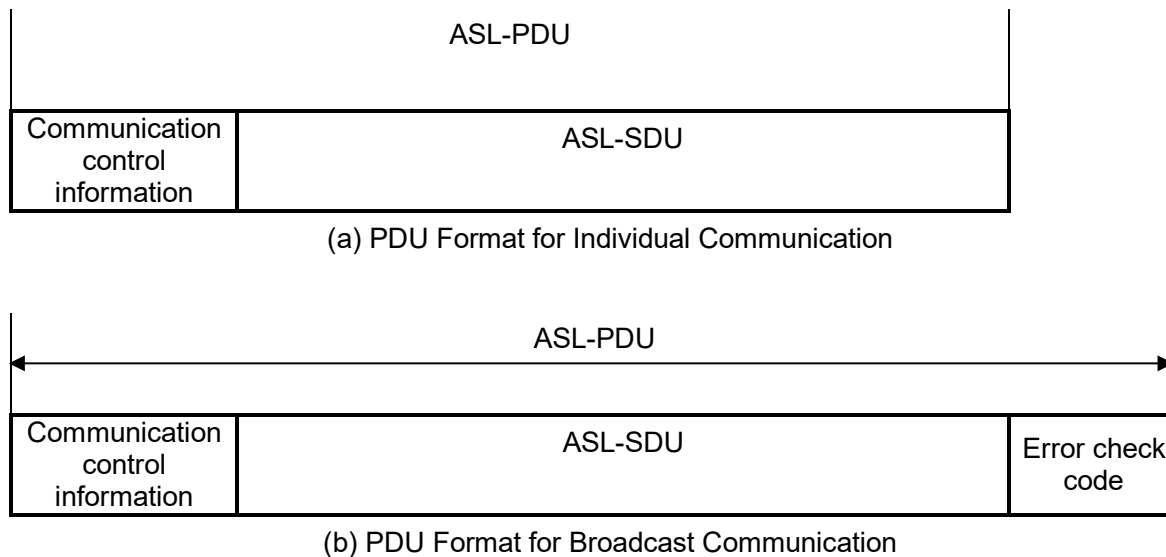
Figure 3.1-5 Configuration of the ASL-PDU (IEEE 802.11/IEEE 802.11bd)
