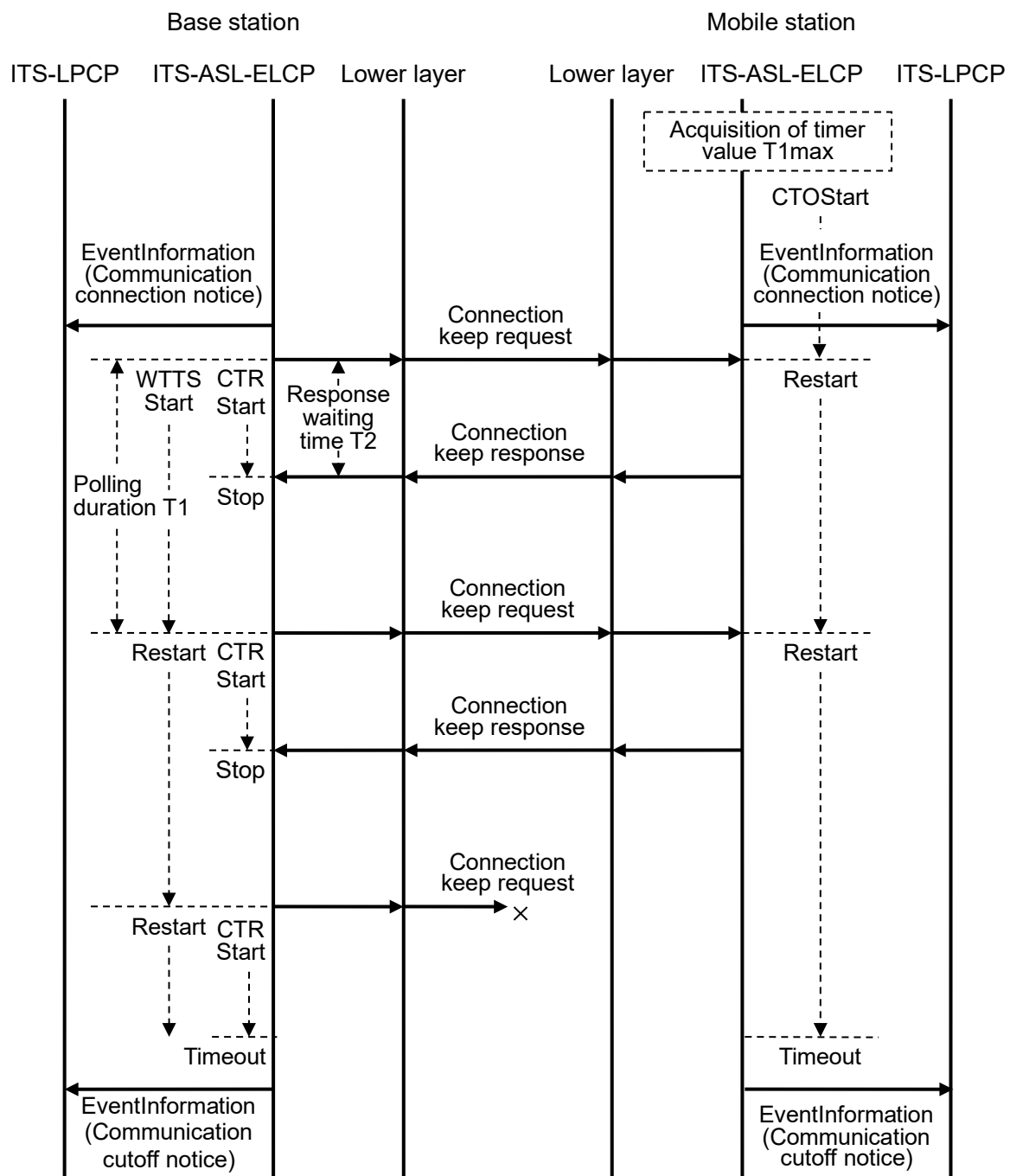
Figure 3.1-14 Example of Communication Connection Management Procedure
