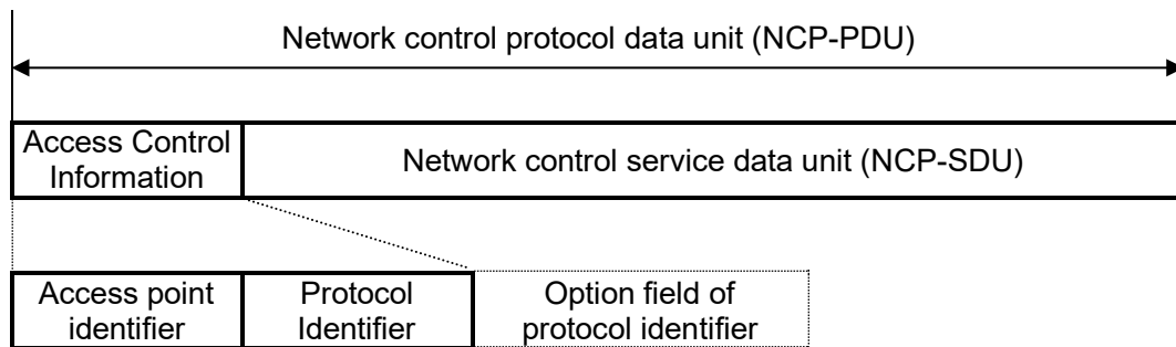
Figure 3.1-12 Communication Control Management PDU Format
