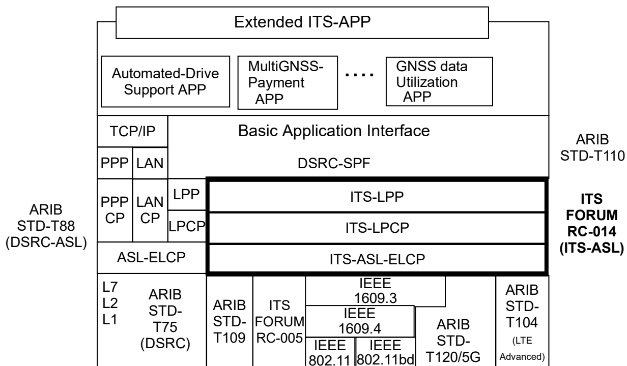
Figure 1.2-1 Protocol configuration of the extended ITS platform
