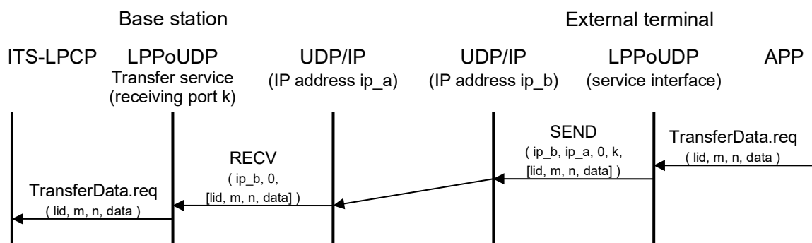
Figure 3.3-32 TransferData.req Sequence
