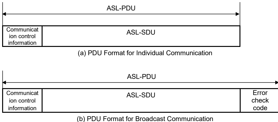
Figure 3.1-7 Configuration of the ASL-PDU (ARIB STD-T109)
