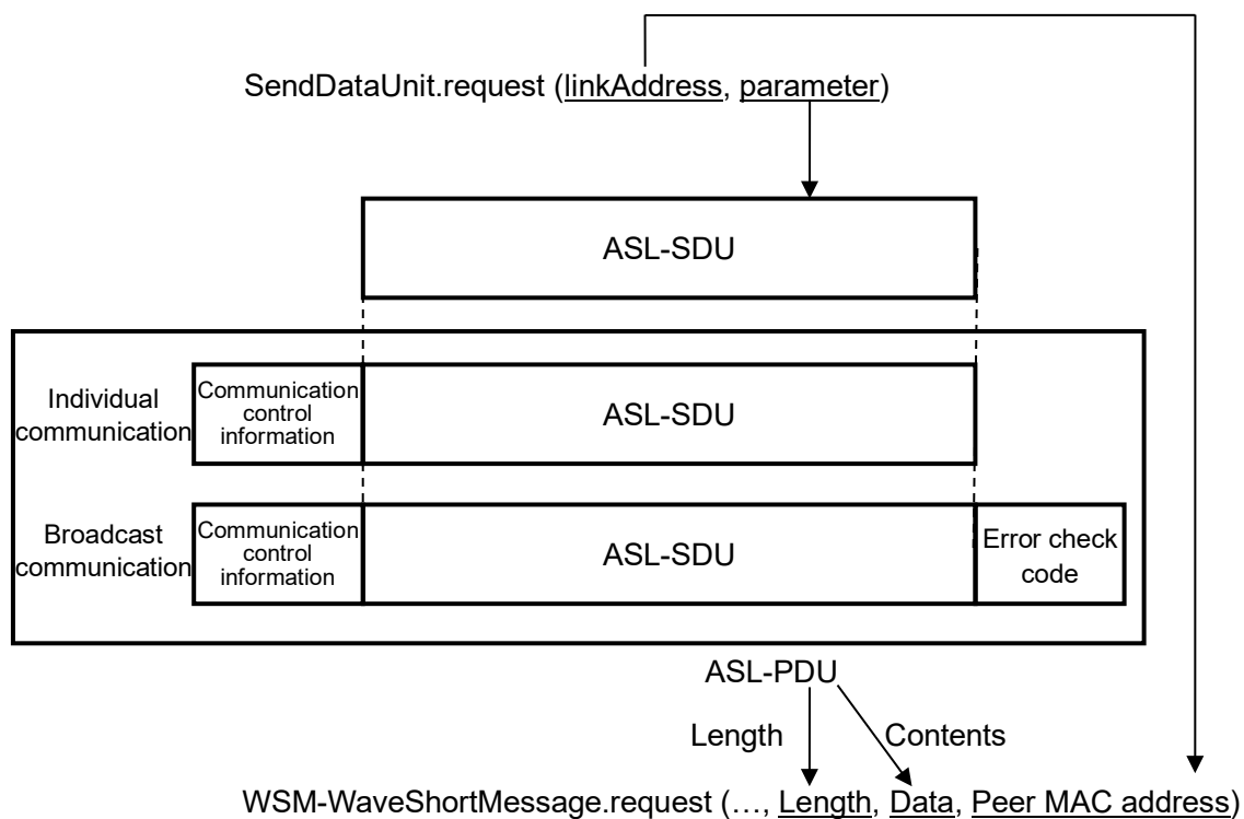
Figure C.3-1 Mapping of sublayer primitive for SendDataUnit.request
