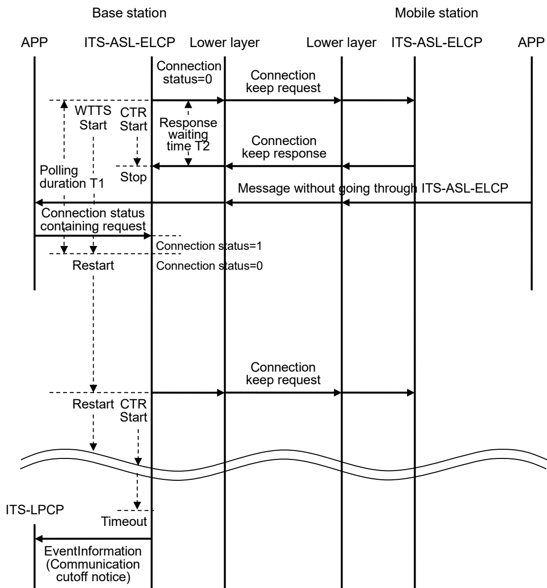
Figure 3.1-16 Example of Communication Connection Management Procedure Set Connection Status by Application
