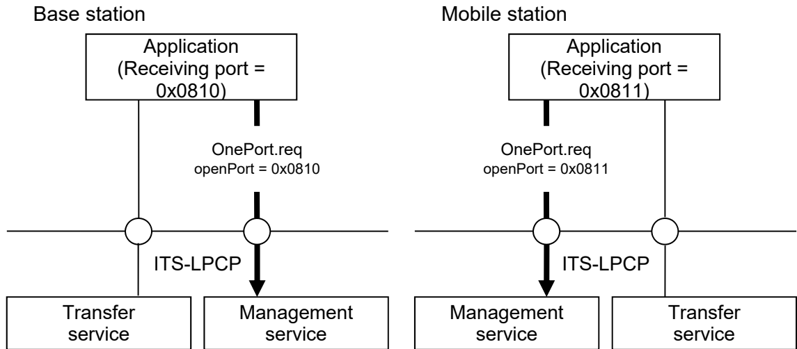
Figure 3.2-14 Example of Application Registration Operation (1)
