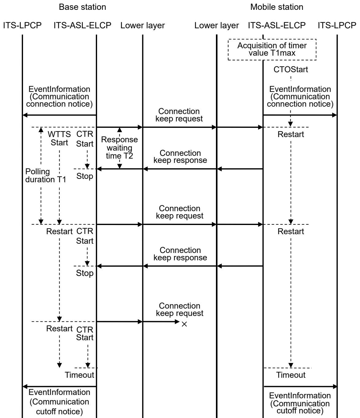
Figure 3.1-12 Example of Communication Connection Management Procedure
