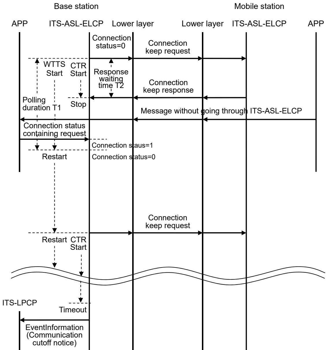
Figure 3.1-14 Example of Communication Connection Management Procedure Set Connection Status by Application
