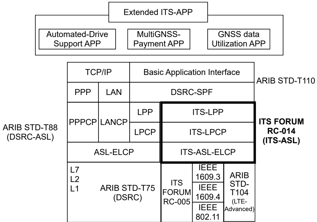
Figure 1.2-1 protocol configuration of the extended DSRC platform
