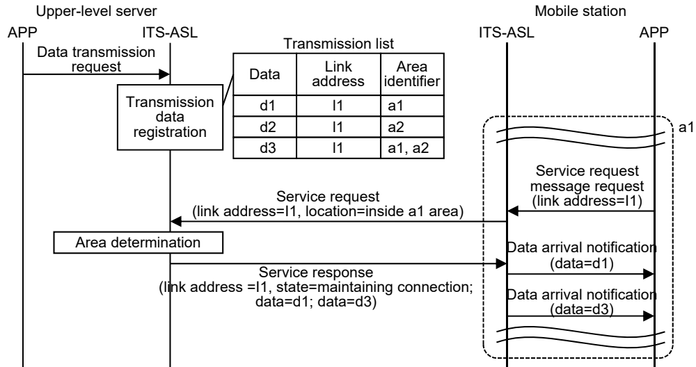
Figure D.7-11 Example of Transmission Service Process Procedure (Driving Inside Single Service Provision Area)
