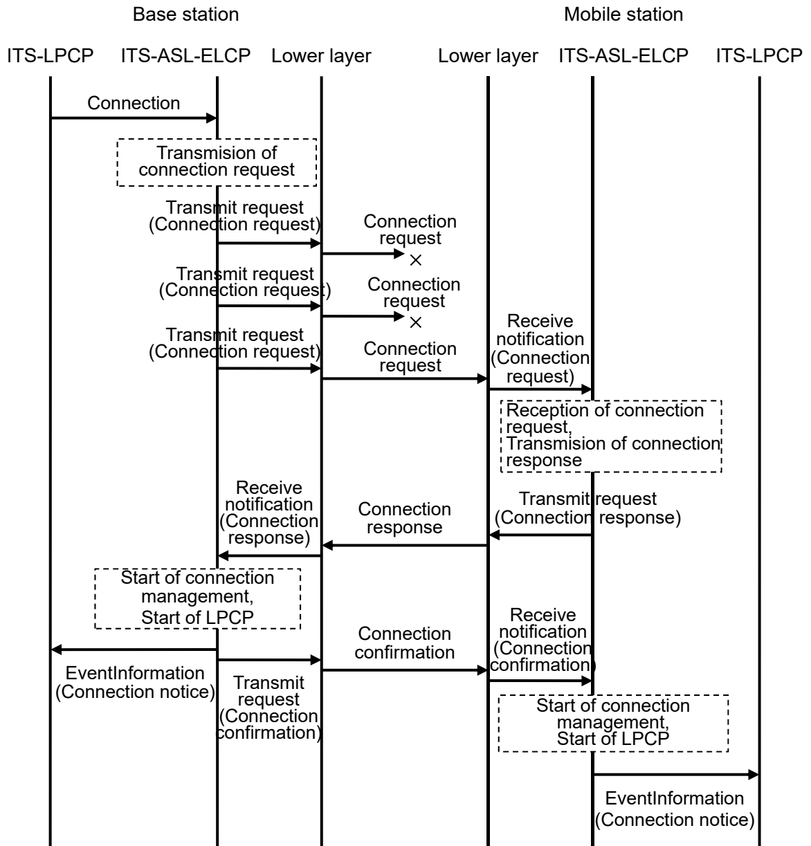
Figure 3.1-11 Example of Communication Connection Procedure
