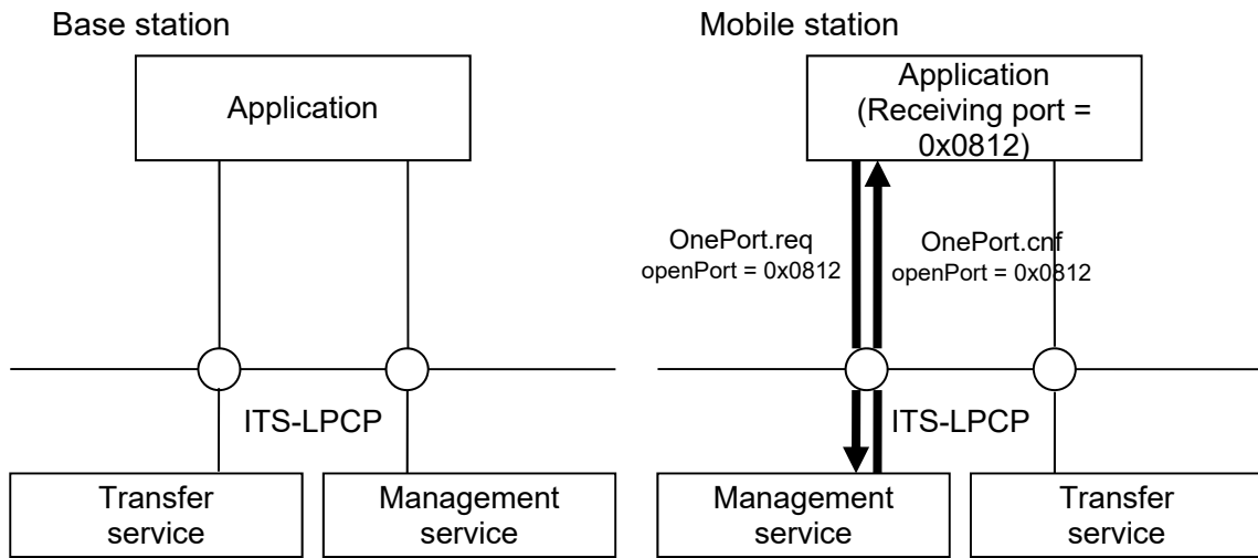
Figure 3.2-20 Application Registration Operation
