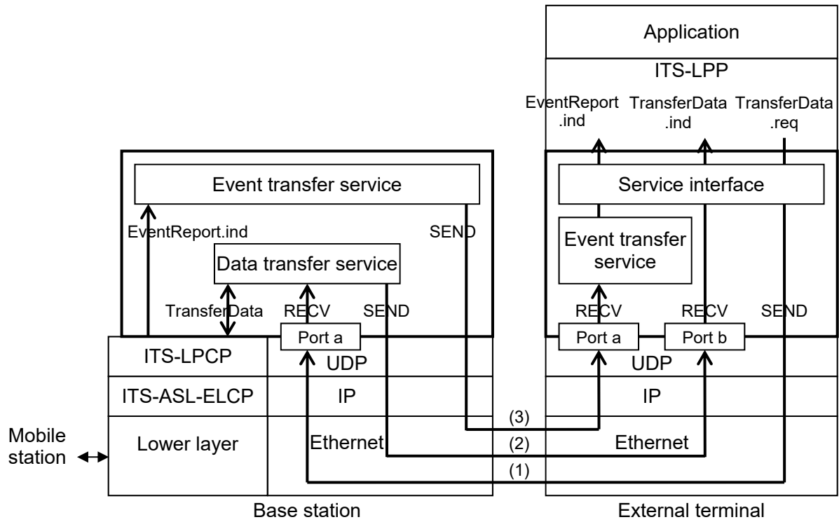
Figure 3.3-28 Outline of LPP over UDP
