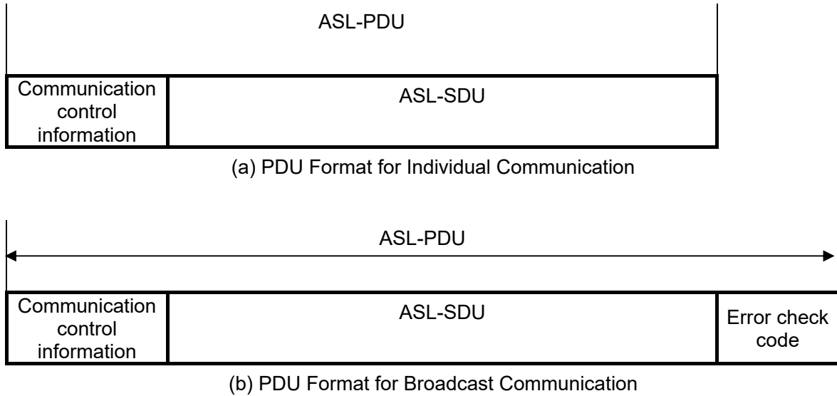
Figure 3.1-5 Configuration of the ASL-PDU (IEEE 802.11)
