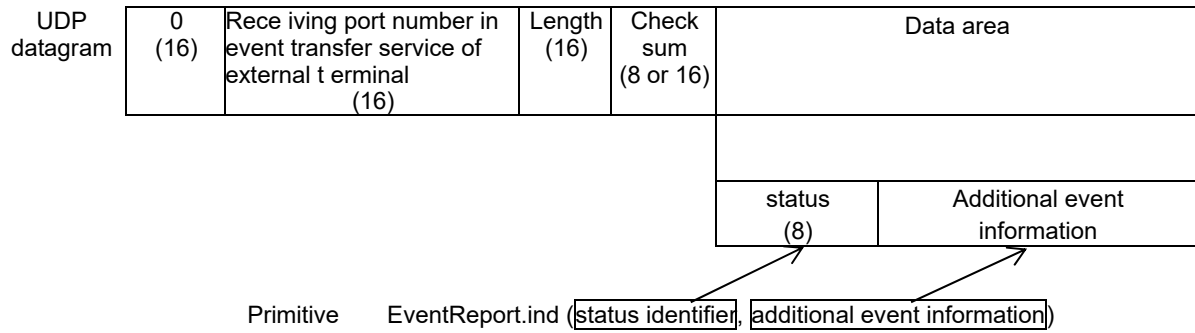
Figure 3.3-35 PDU Mapping in EventReport.ind
