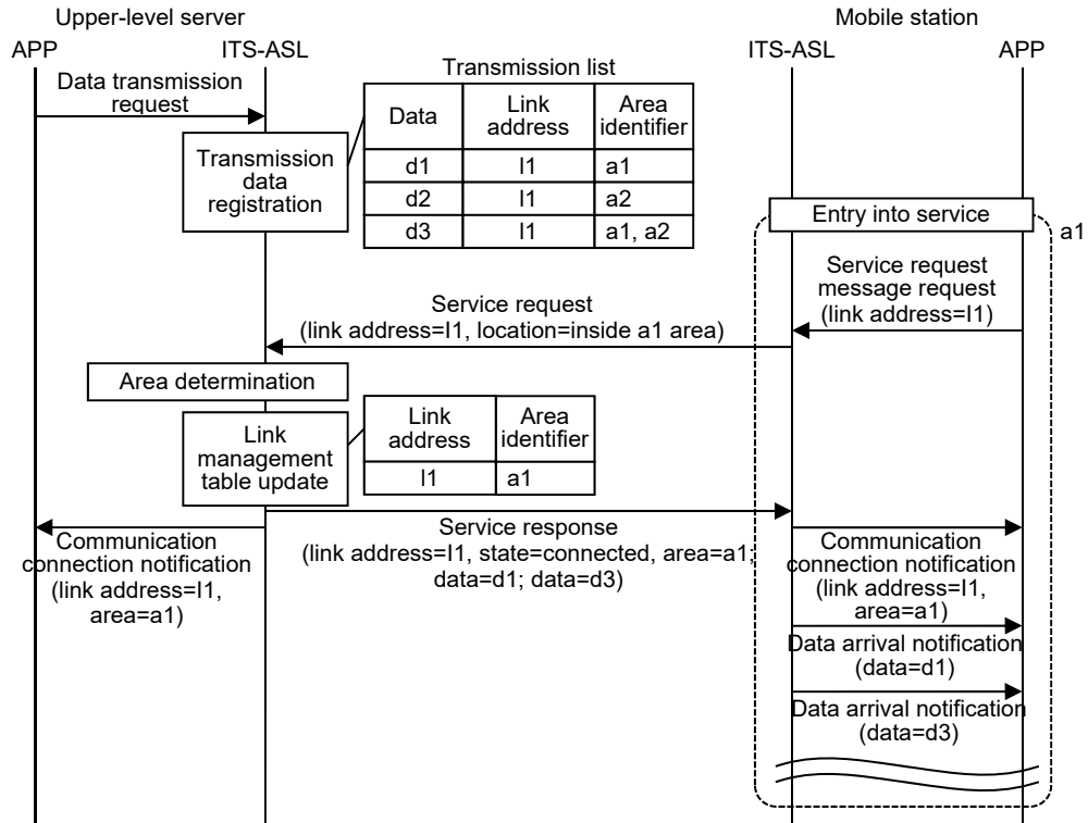
Figure D.7-13 Example of Transmission Service Process Procedure (Entering Service Provision Area)
