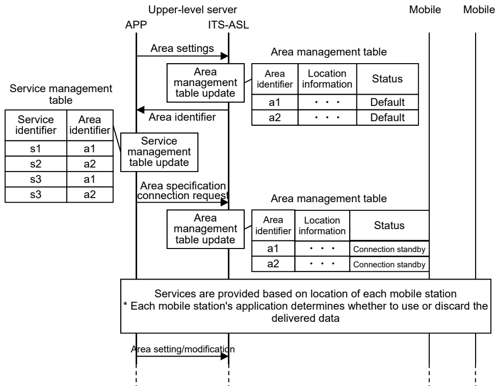
Figure D.7-2 Example of Management Procedure for Services and Service Provision Areas
