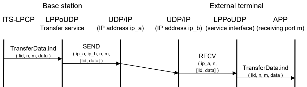
Figure 3.3-34 TransferData.ind Sequence
