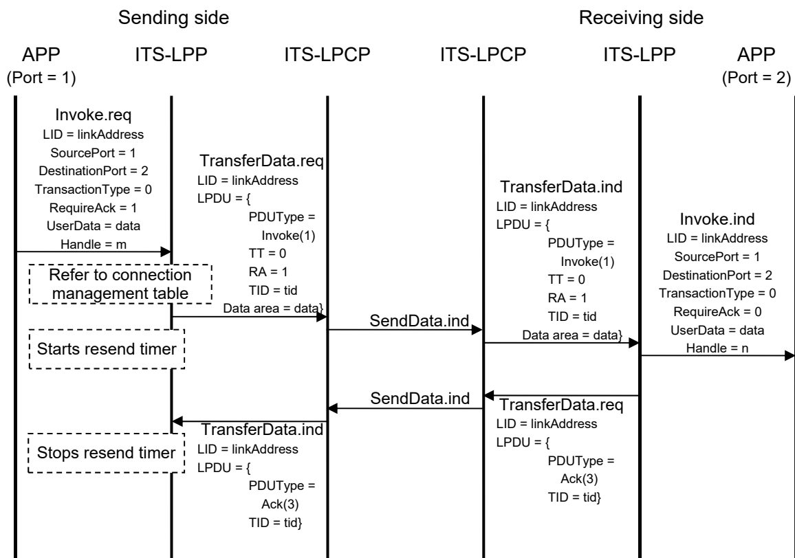
Figure 3.3-17 Example of Resend Processing (Basic sequence)
