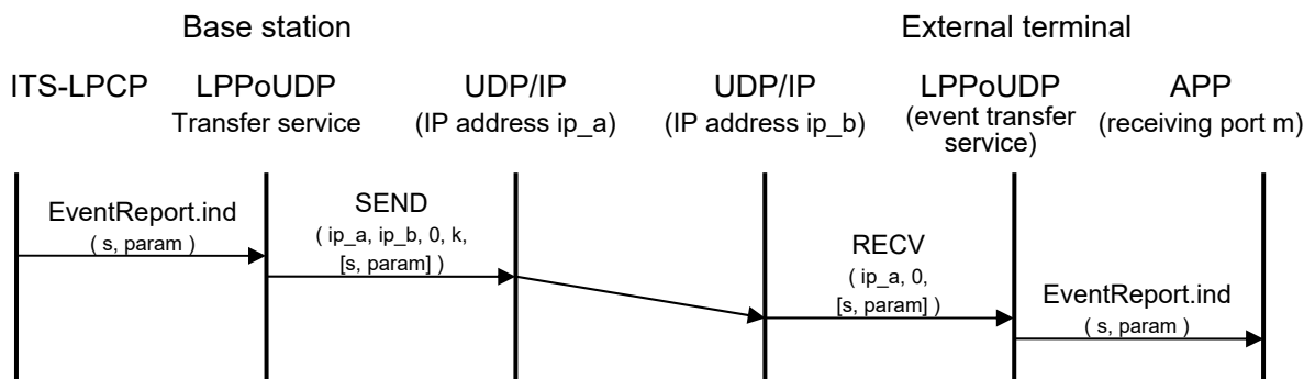
Figure 3.3-36 EventReport.ind Sequence
