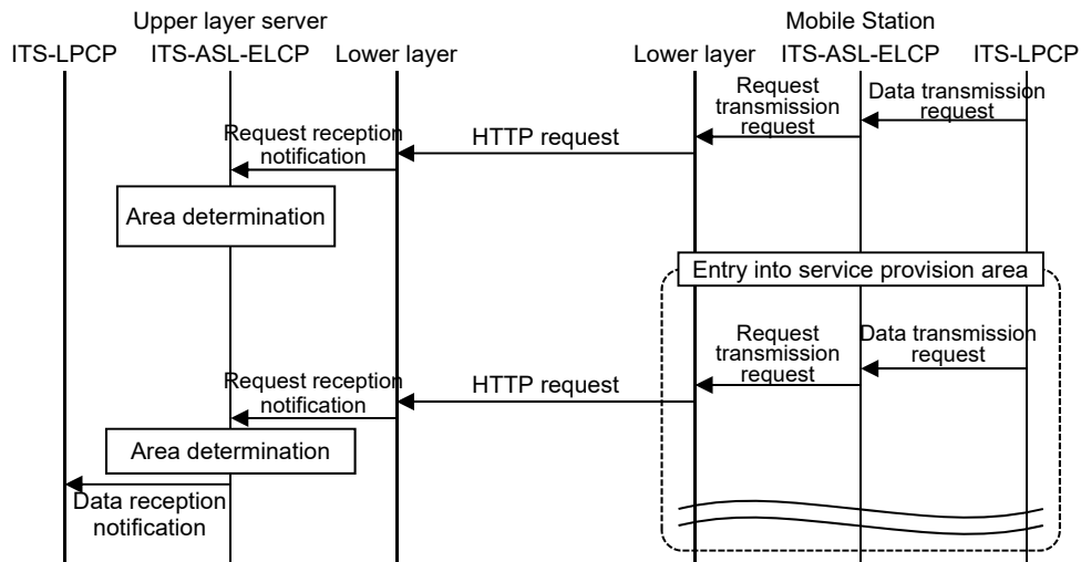
Figure 3.1-7 Example of Mobile Station to Upper Layer Server Data Transfer Service Process Procedure
