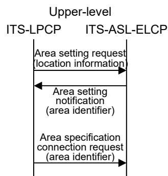
Figure 3.1-15 Example of Area Setting Procedure
