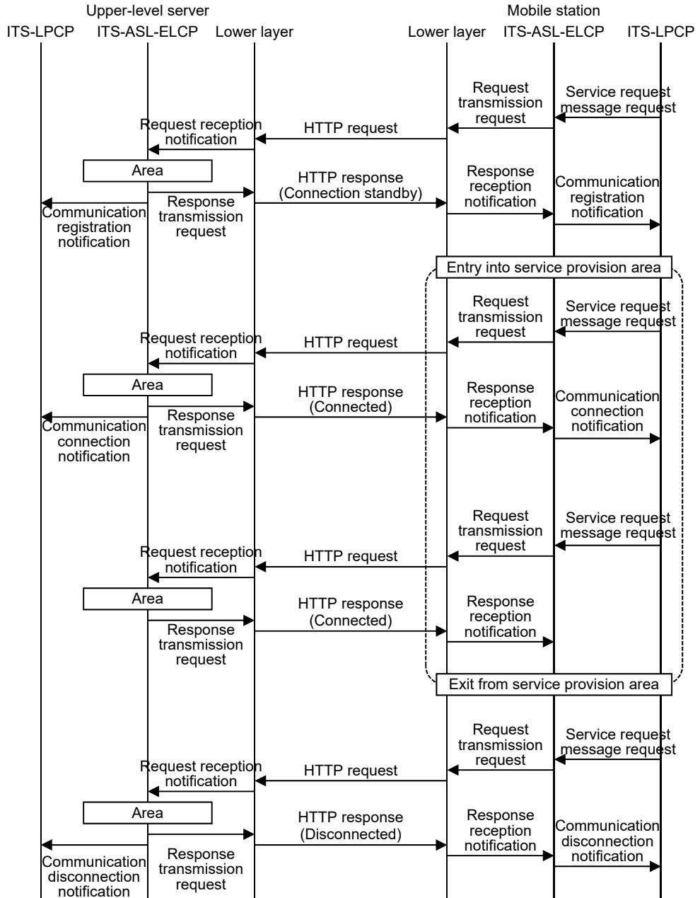
Figure 3.1 16 Example of Communication Connection Procedure
