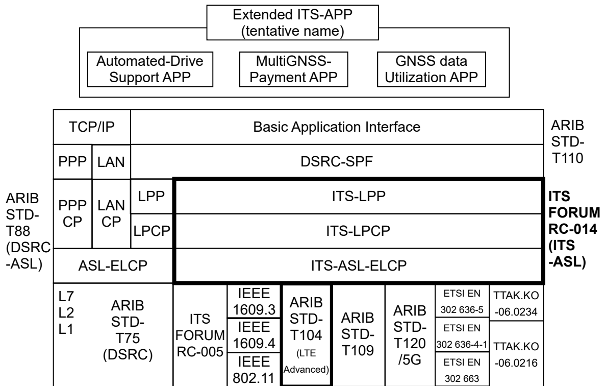
FigureA.2-1 protocol configuration of the extended DSRC platform
