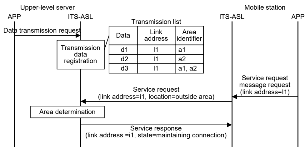
Figure D.7-10 Example of Transmission Service Process Procedure (Driving Outside Service Provision Area)
