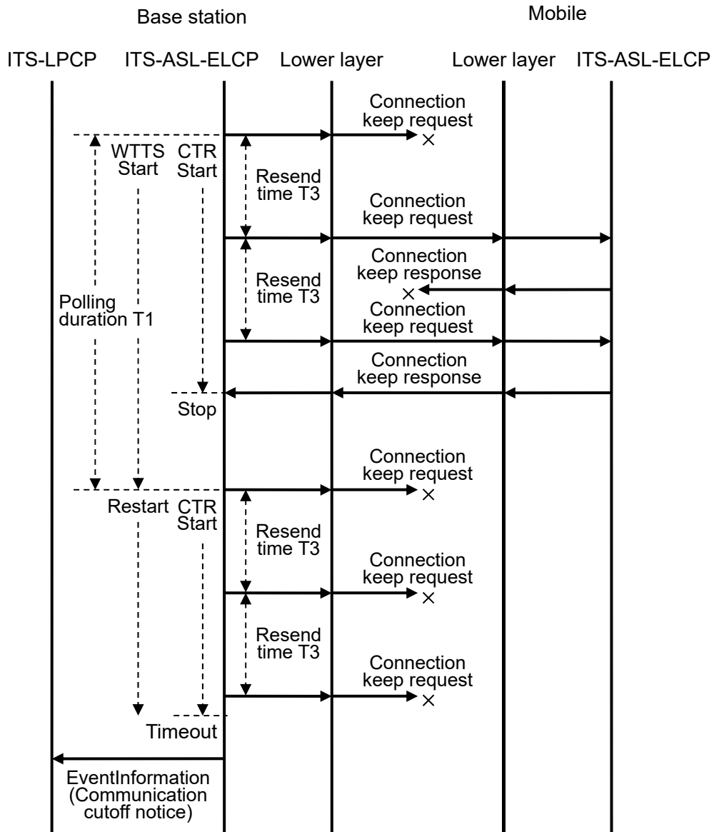
Figure 3.1-13 Example of Resend Control Procedure of Connection Keep Request
