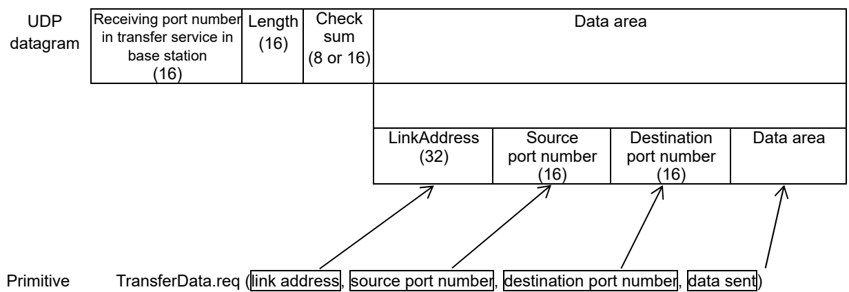
Figure 3.3-31 PDU Mapping in TransferData.req
