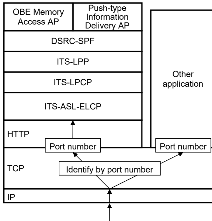
Figure 2.2-3 Identification of the Destination Application in ARIB STD-T104
