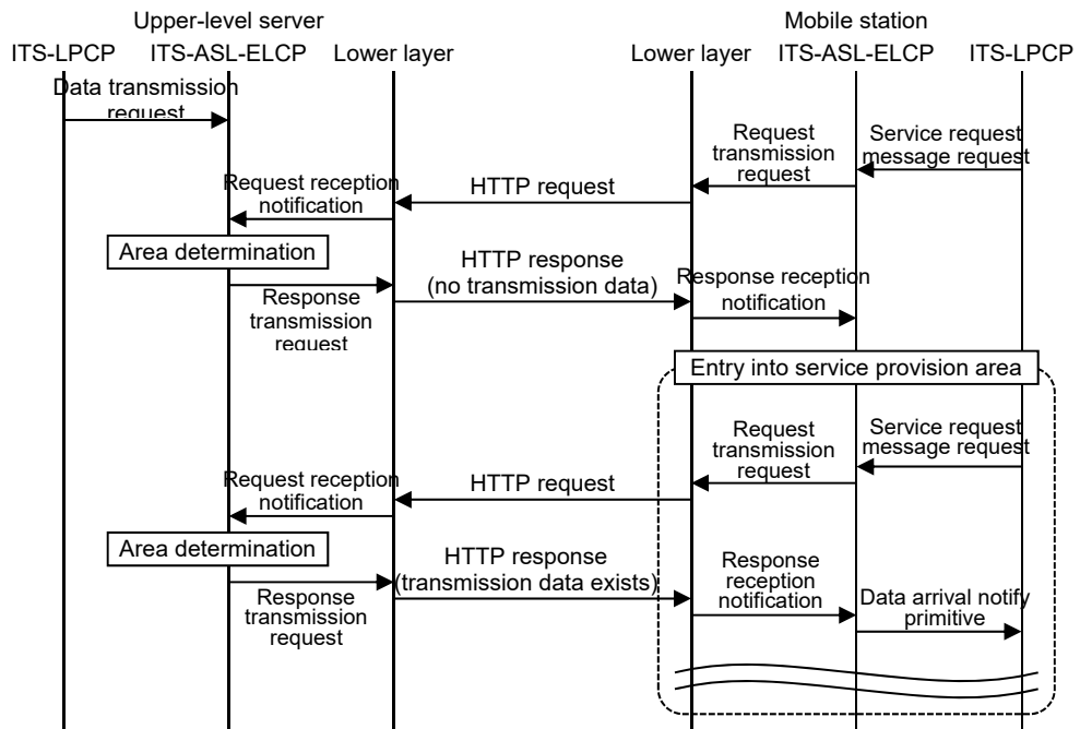
Figure 3.1-8 Example of Upper Layer Server to Mobile Station Data Transfer Service Process Procedure
