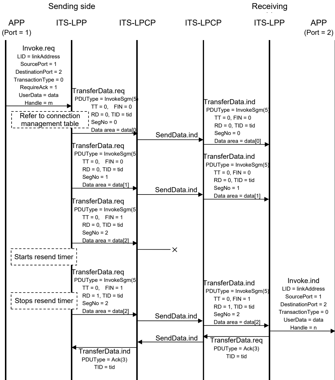
Figure 3.3-22 Example of Segmentation/re-assembly Process (When final segment data have not been received)
