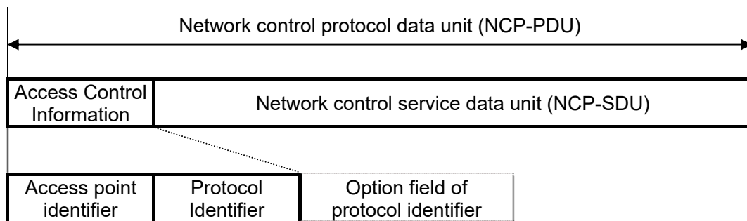
Figure 3.1-10 Communication Control Management PDU Format
